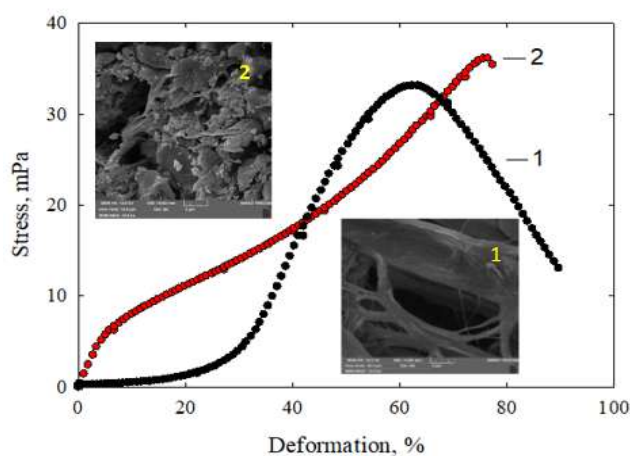
Fig. 1. Deformation and SEM images of the pristine (1) and modified (2) membranes.
