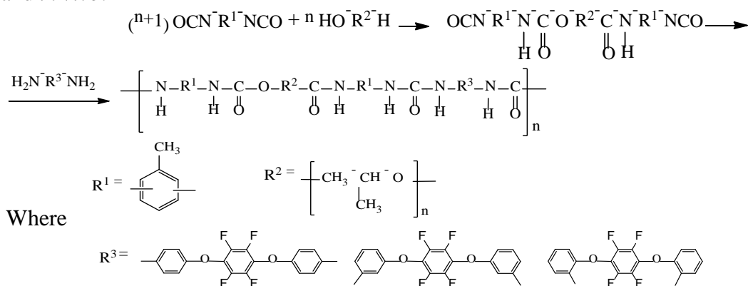
Fig. Reaction scheme synthesis of FPUUs.
